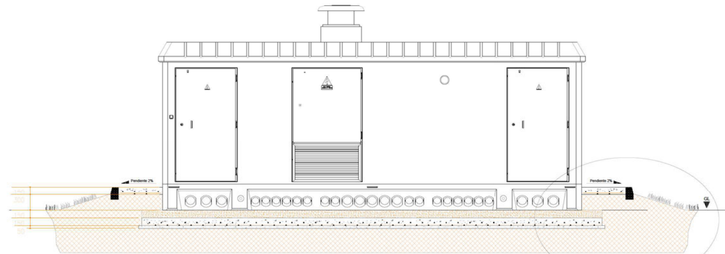
VISTA FRONTAL
