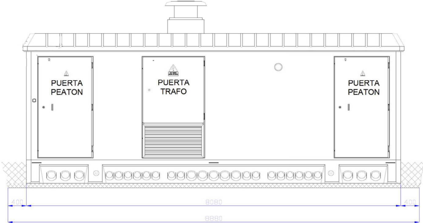
VISTA FRONTAL
